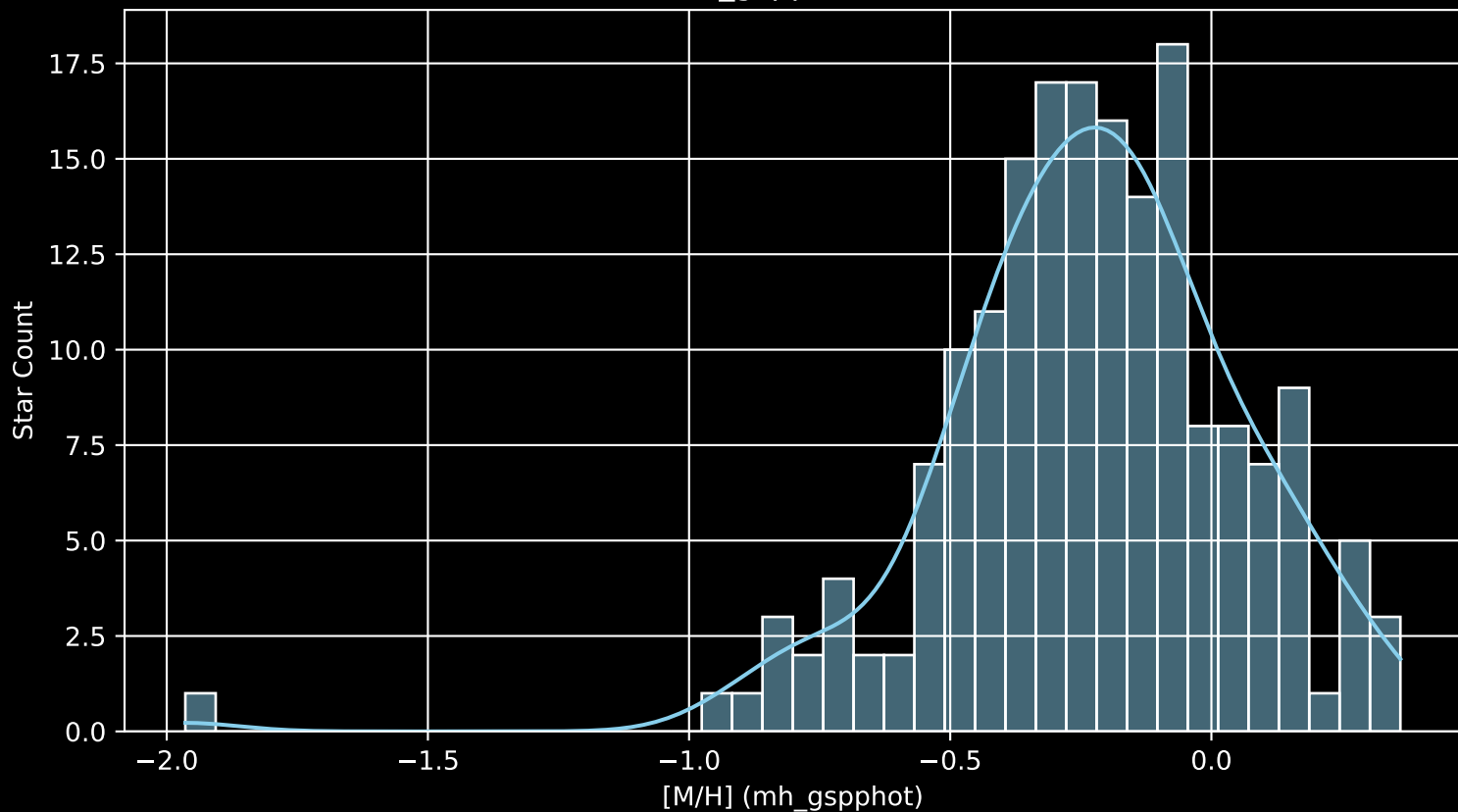
APOGEE DR17 Field: [133+76_MGA [M/H] (mh_gspphot) (n= 182)
