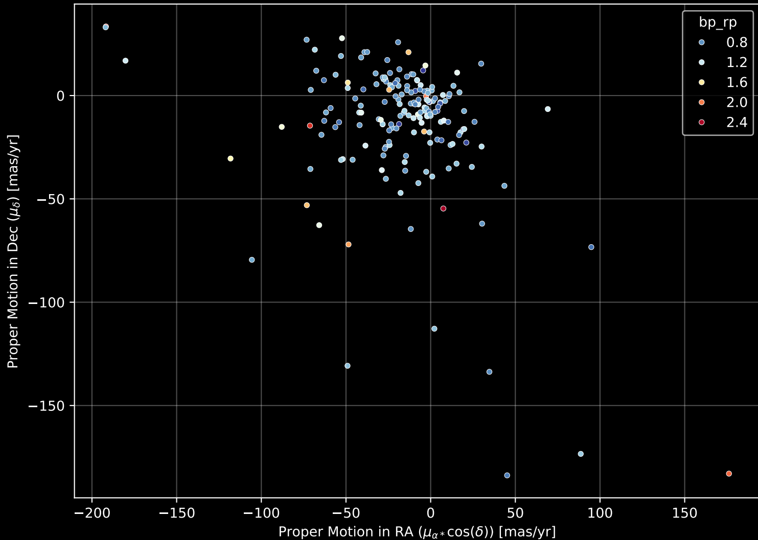
APOGEE DR17 Field: [133+76_MGA] Proper Motion Diagram (n= 183)
