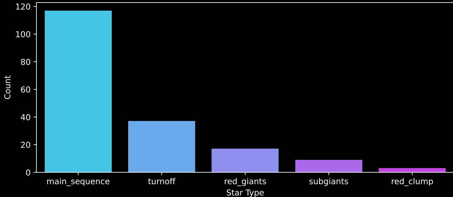
APOGEE DR17 Field: [133+76_MGA] Count plot of Star Type
