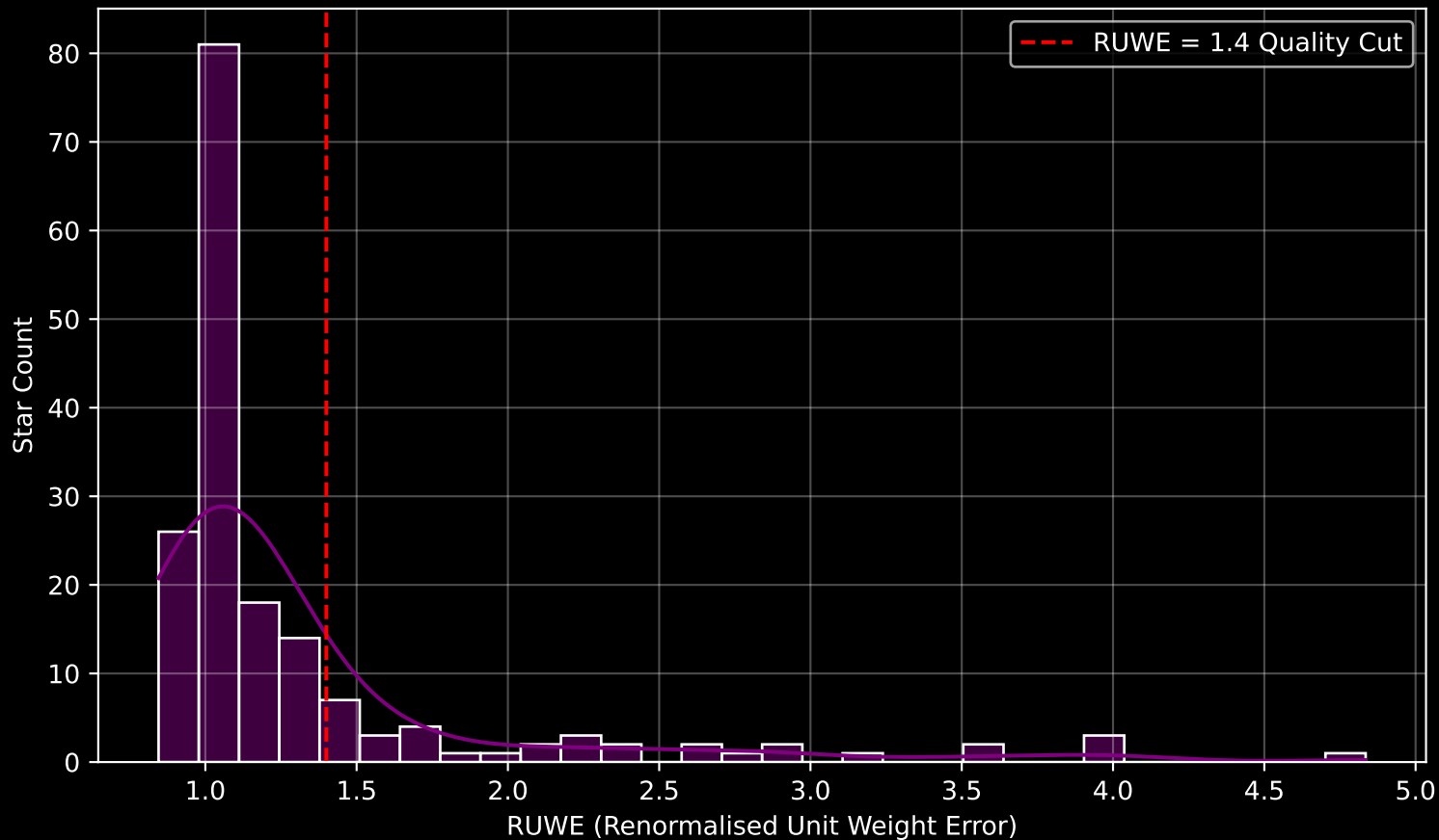
GAPOGEE DR17 Field [133+76_MGA] RUWE Distribution (n= 174)
