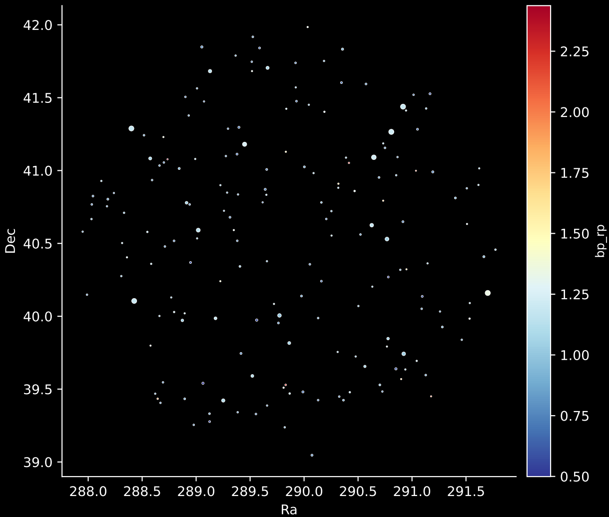
APOGEE DR17 Field: [133+76_MGA] Stars: 183
