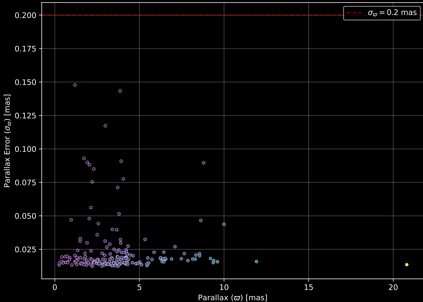
APOGEE DR17 Field: [133+76_MGA] Parallax Quality (n= 183)
